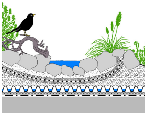
Floradrain® FD 25-E
